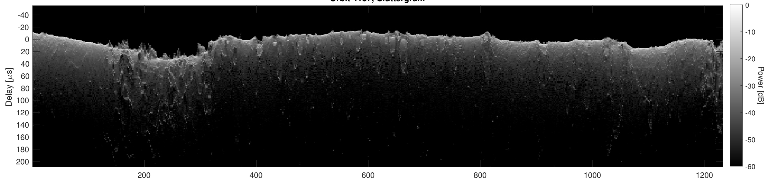
Orbit 4137, Cluttergram
