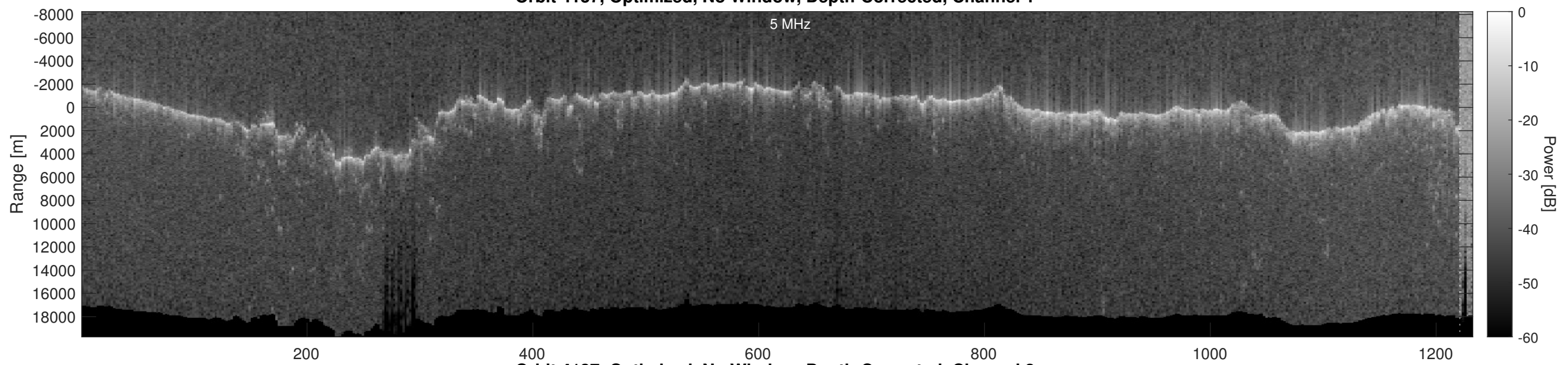
Orbit 4137, Optimized, No Window, Depth-Corrected, Channel 2
