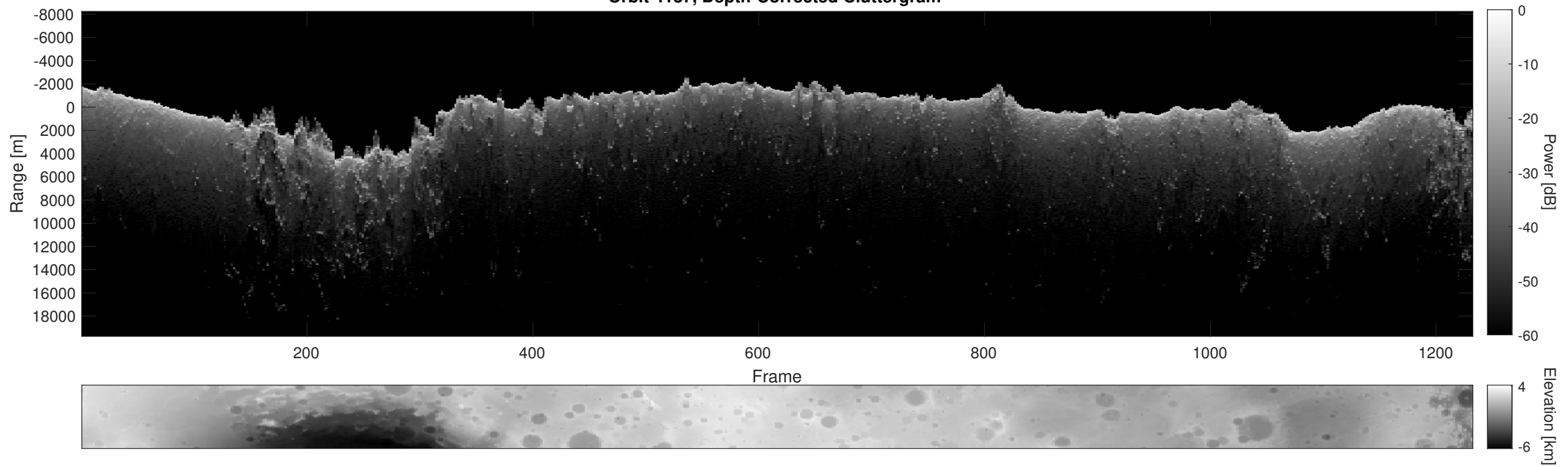
Orbit 4137, Depth-Corrected Cluttergram
