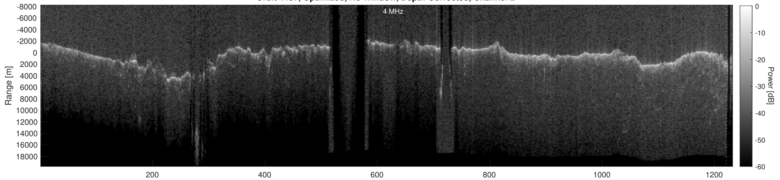
Orbit 4137, Depth-Corrected Cluttergram
