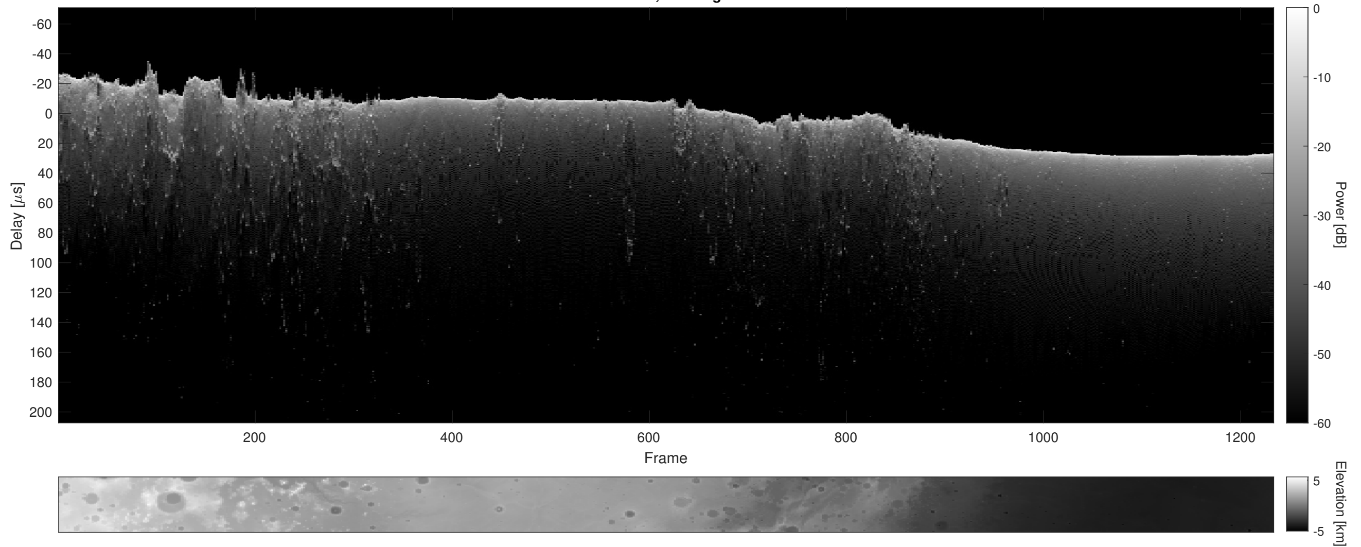
Orbit 4140, Cluttergram
