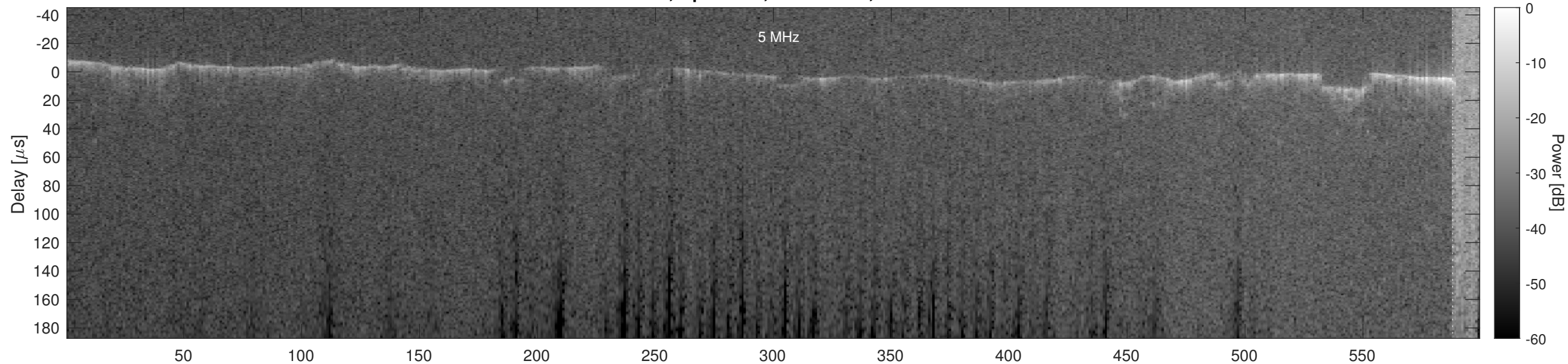
Orbit 4141, Optimized, No Window, Channel 2
