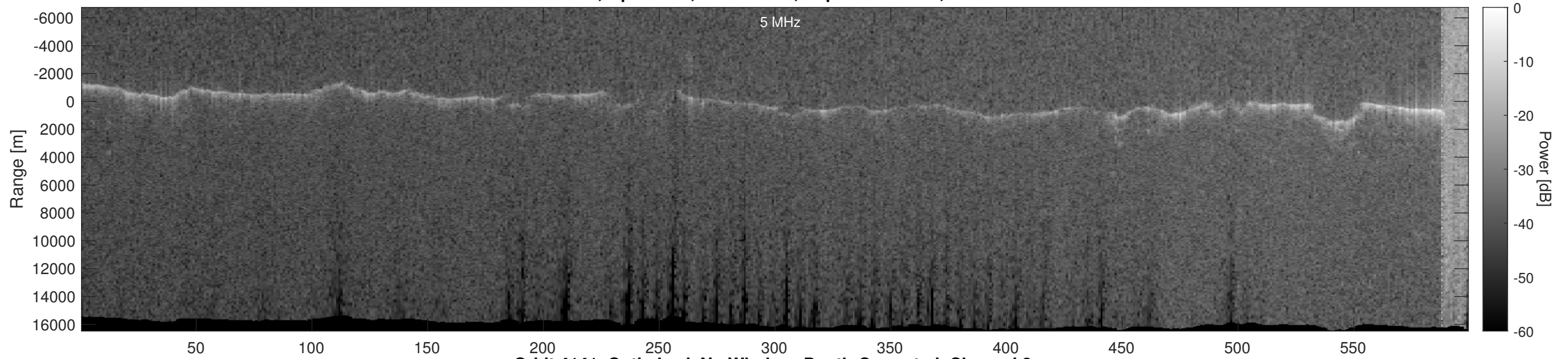
Orbit 4141, Optimized, No Window, Depth-Corrected, Channel 2
