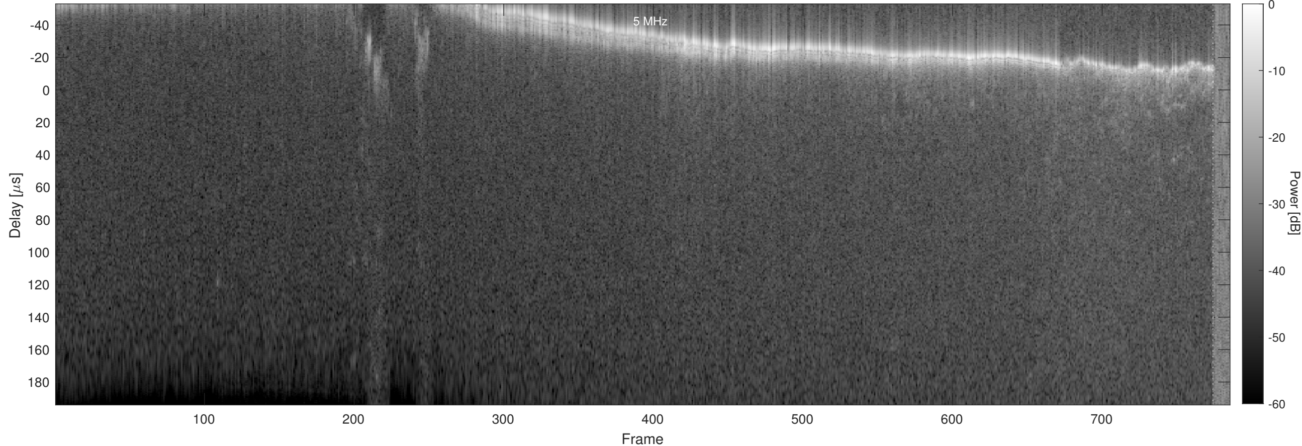
Orbit 4142, Chapman, No Window, Channel 2
