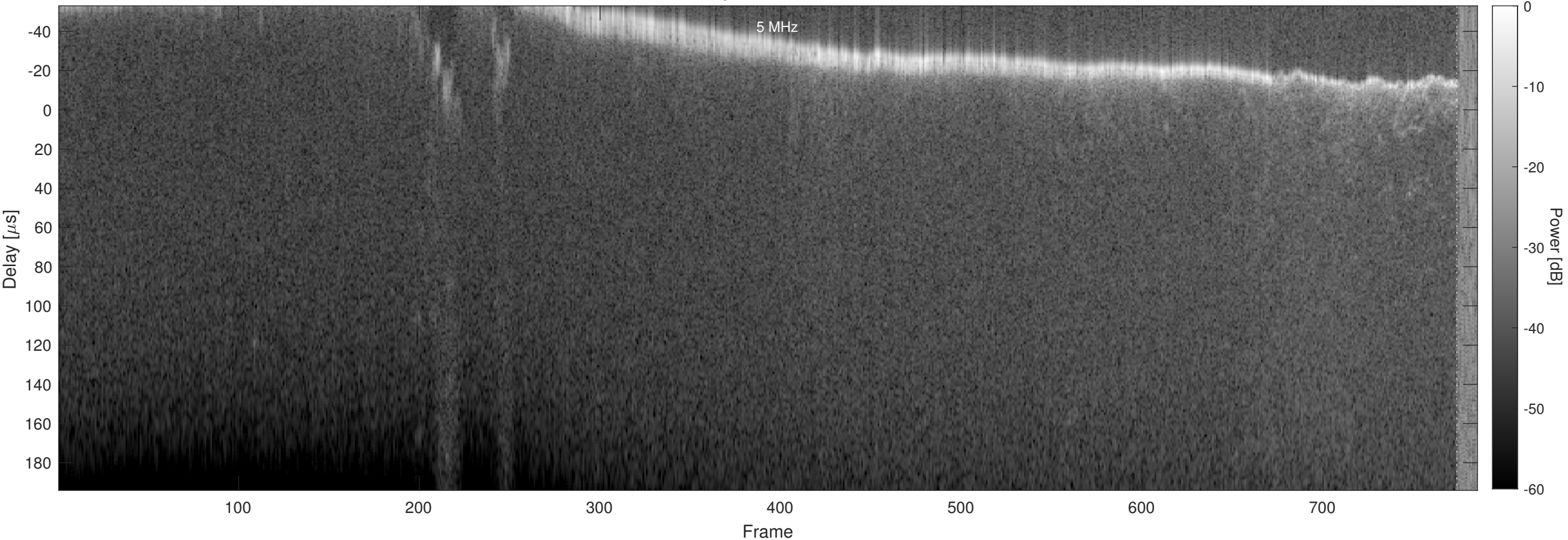
Orbit 4142, Chapman, Window, Channel 2
