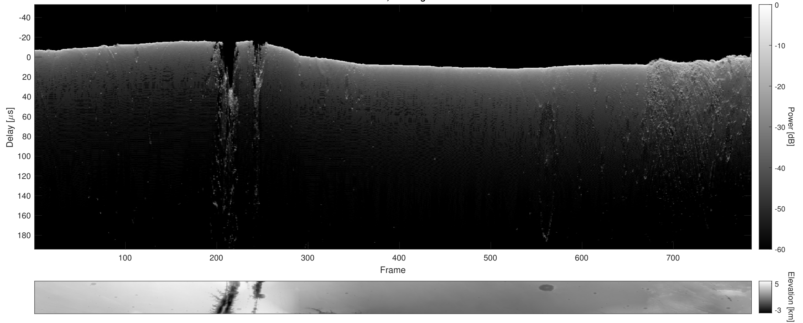
Orbit 4142, Cluttergram
