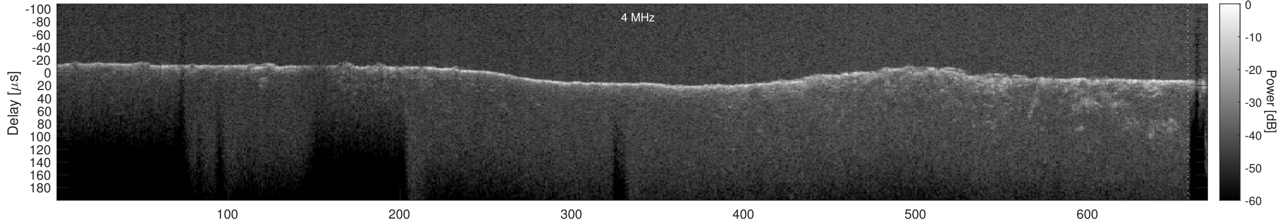
Orbit 4144, Cluttergram
