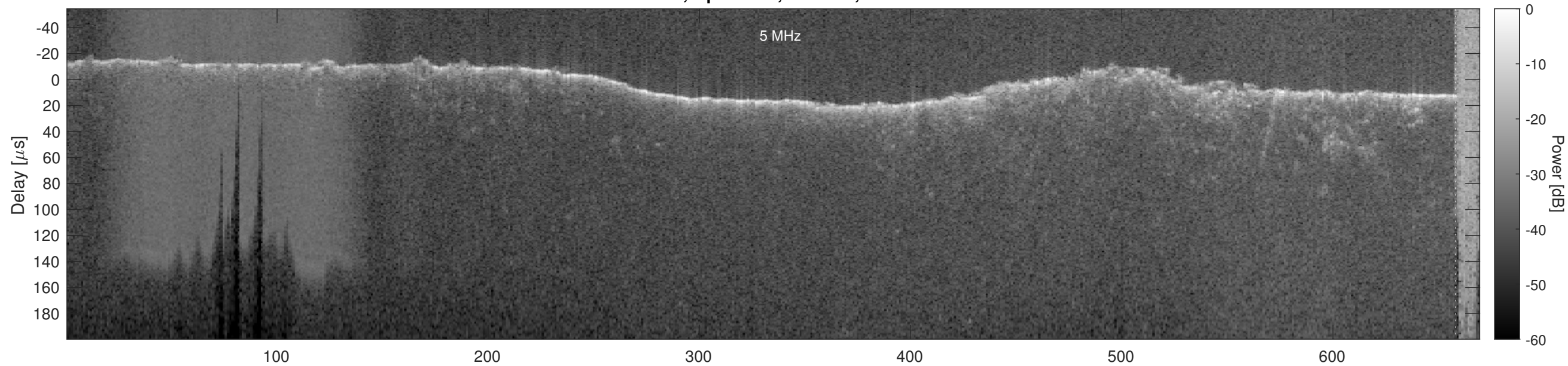
Orbit 4144, Optimized, Window, Channel 2
