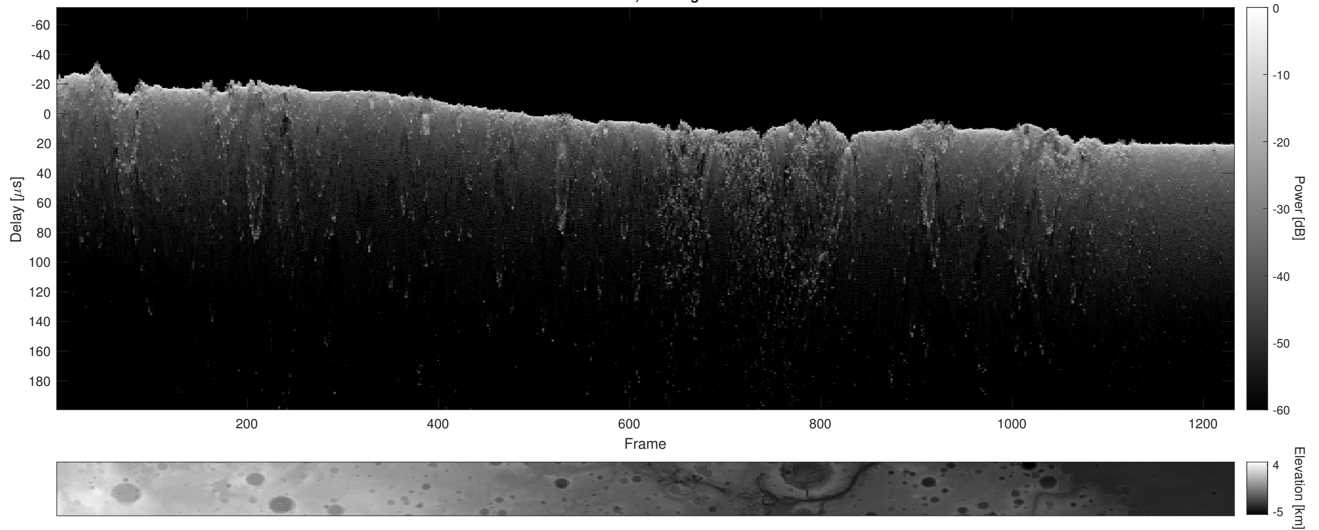
Orbit 4145, Cluttergram
