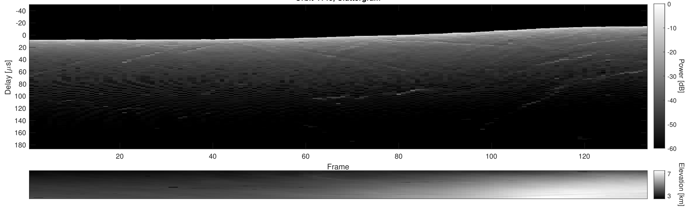
Orbit 4146, Cluttergram
