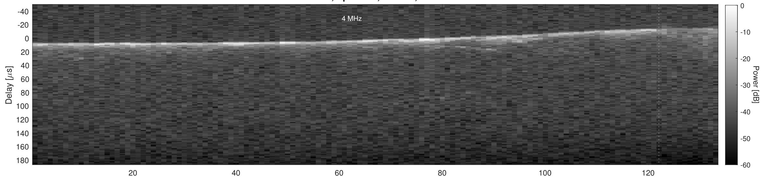
Orbit 4146, Cluttergram
