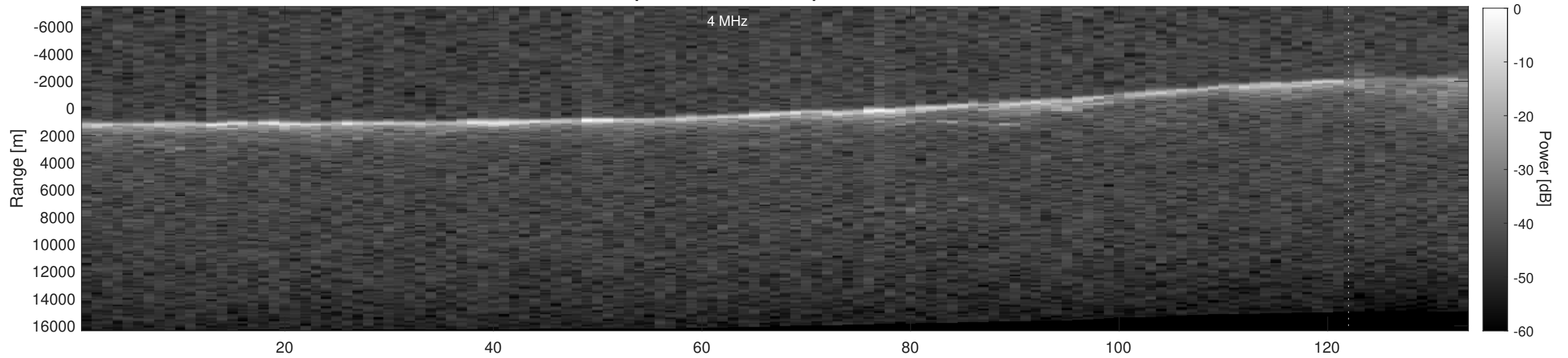
Orbit 4146, Depth-Corrected Cluttergram
