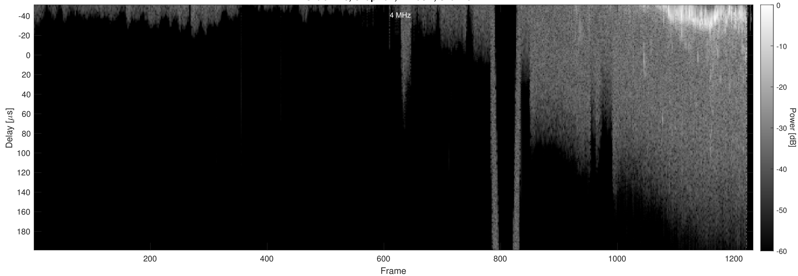
Orbit 4148, Chapman, Window, Channel 2
