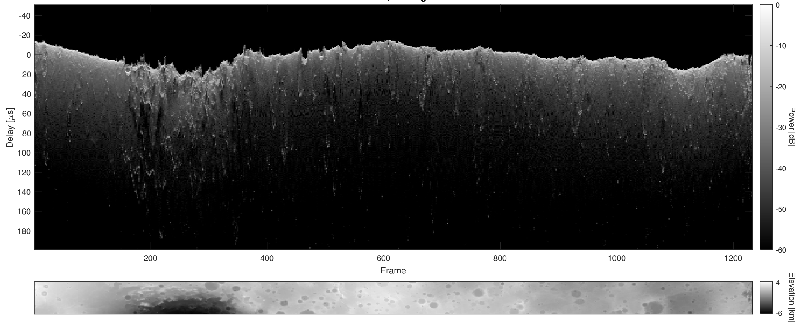
Orbit 4148, Cluttergram
