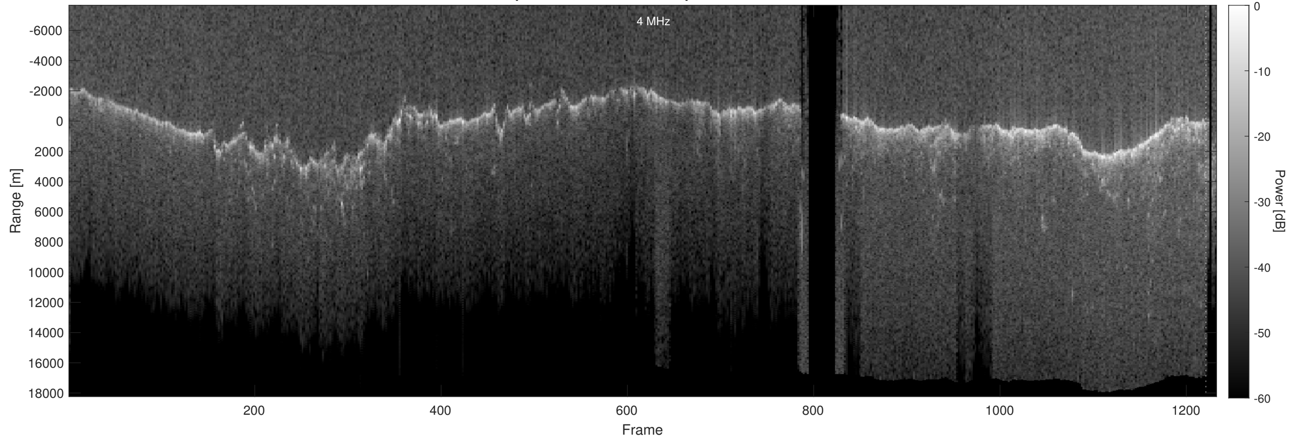
Orbit 4148, Optimized, No Window, Depth-Corrected, Channel 2
