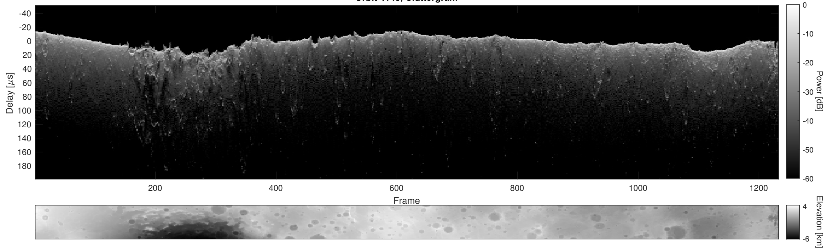
Orbit 4148, Cluttergram
