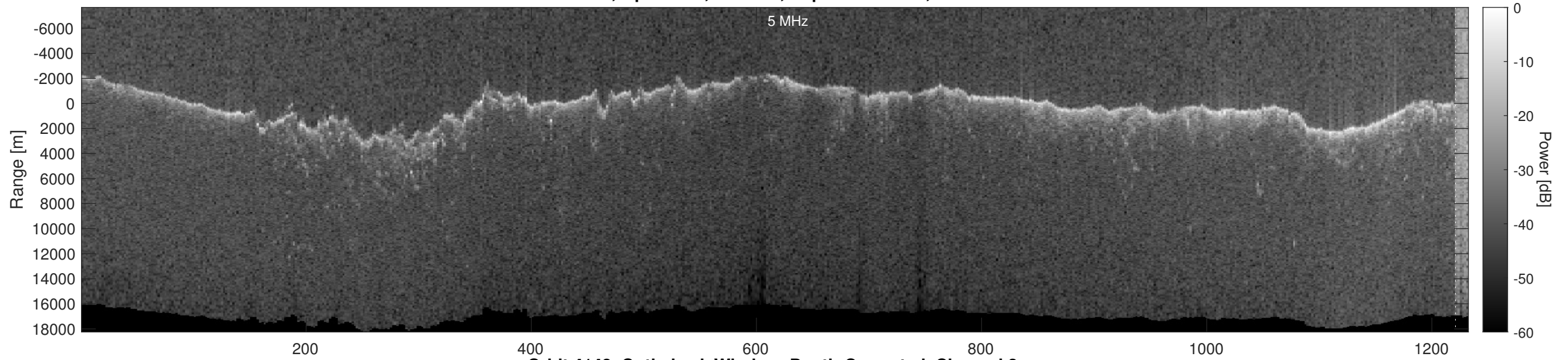
Orbit 4148, Optimized, Window, Depth-Corrected, Channel 2
