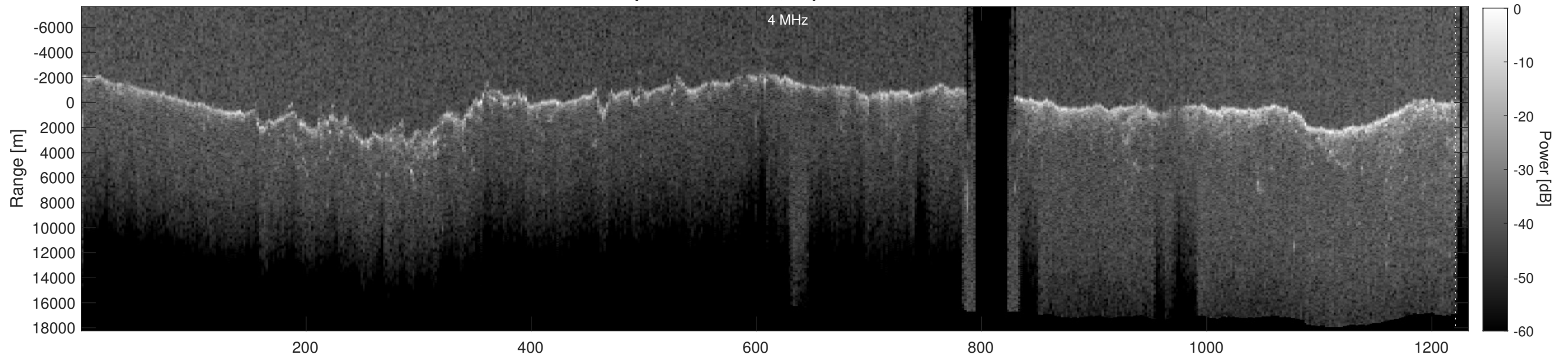
Orbit 4148, Depth-Corrected Cluttergram
