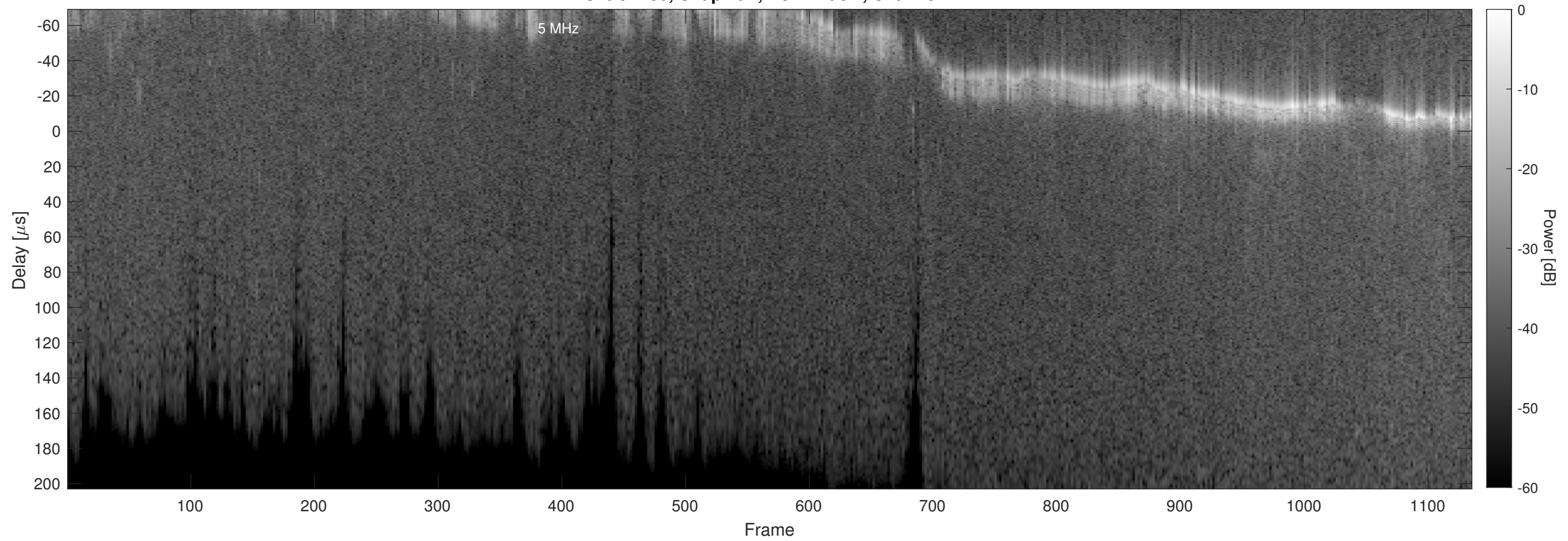
Orbit 4150, Chapman, No Window, Channel 2
