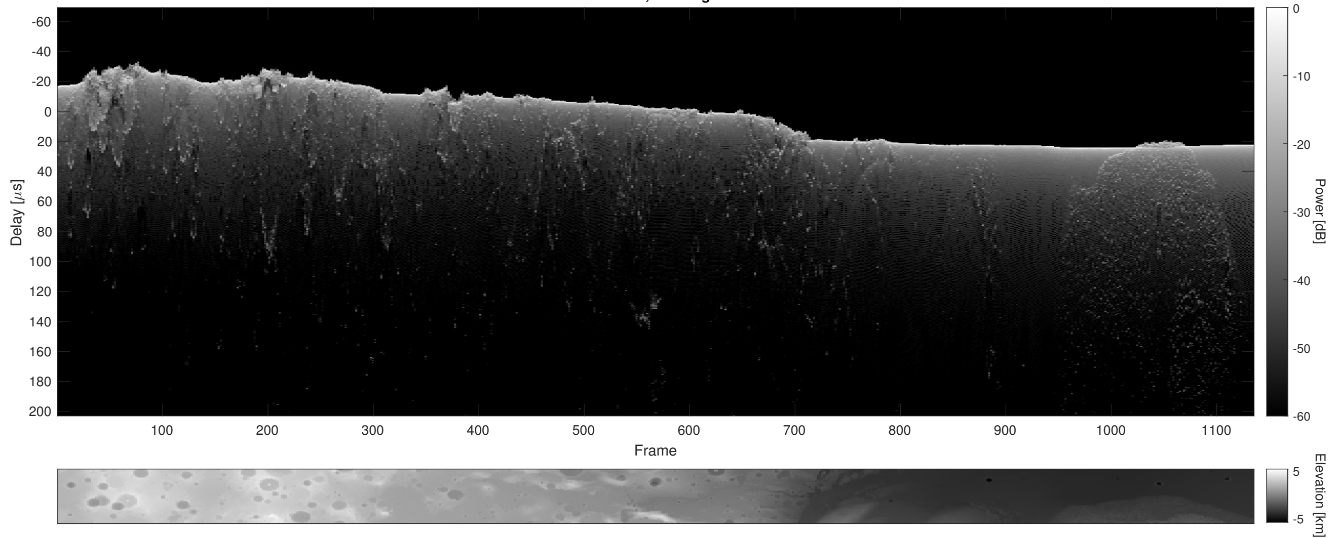
Orbit 4150, Cluttergram
