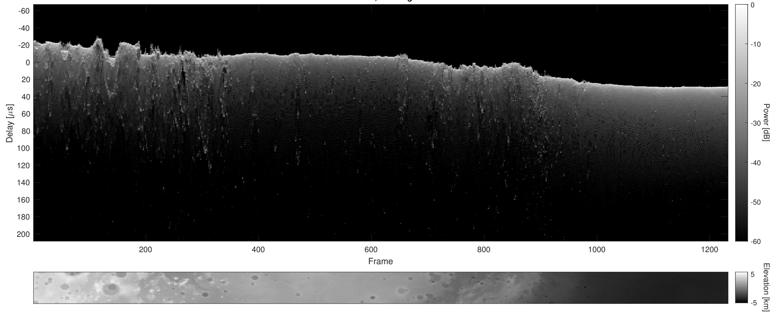
Orbit 4151, Cluttergram
