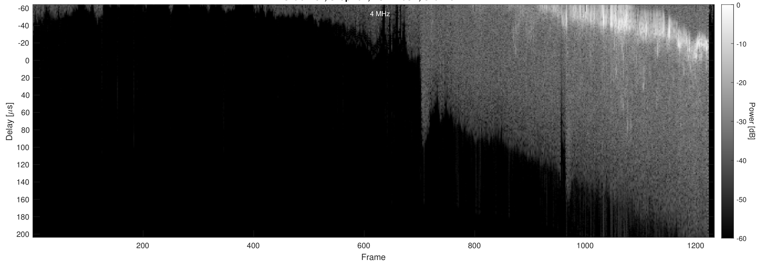
Orbit 4152, Chapman, No Window, Channel 2
