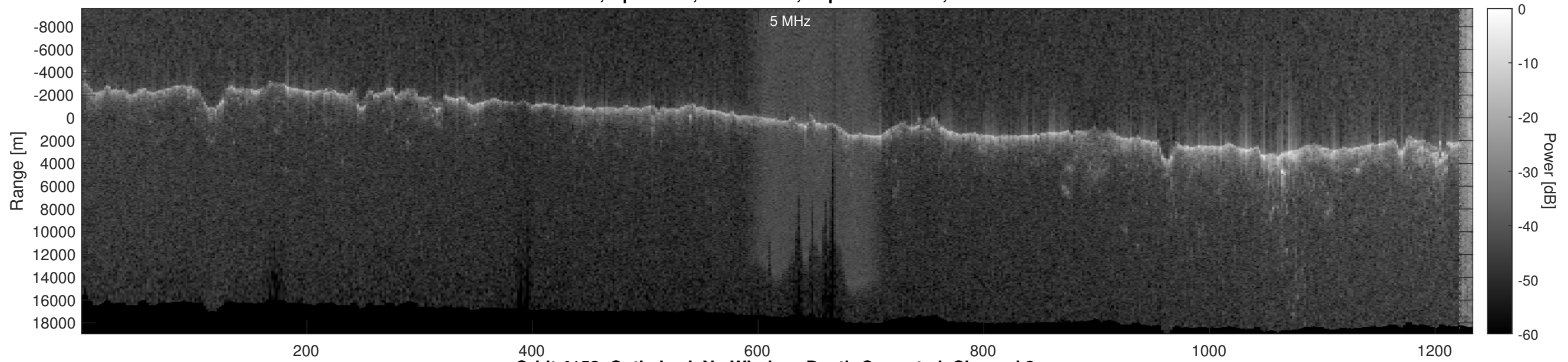
Orbit 4152, Optimized, No Window, Depth-Corrected, Channel 2
