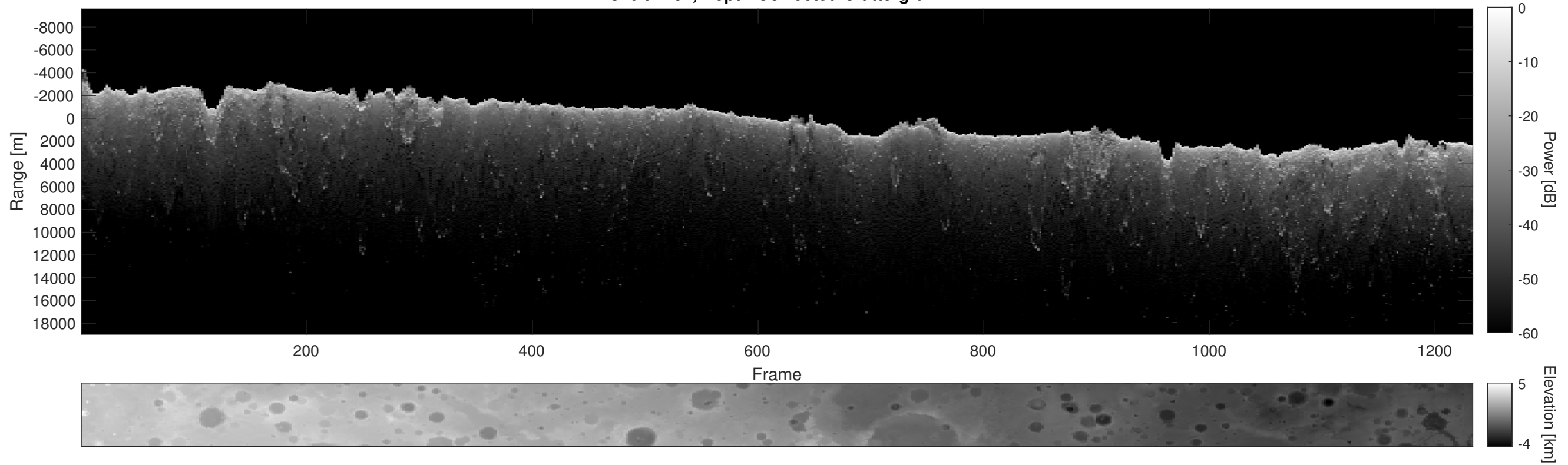
Orbit 4152, Depth-Corrected Cluttergram
