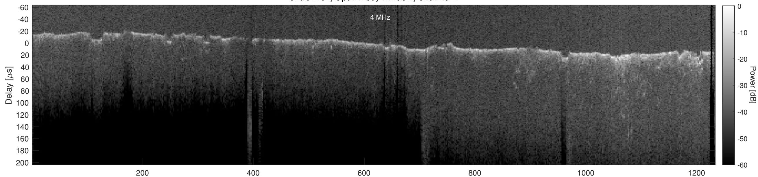
Orbit 4152, Cluttergram
