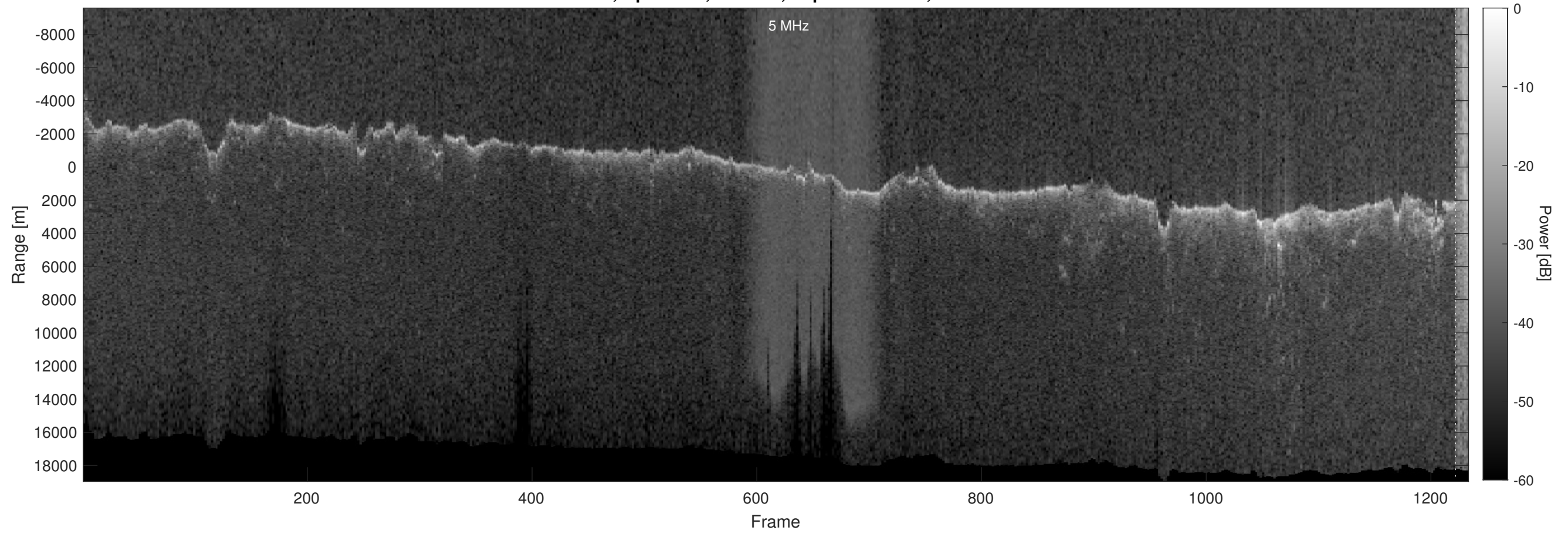
Orbit 4152, Optimized, Window, Depth-Corrected, Channel 2
