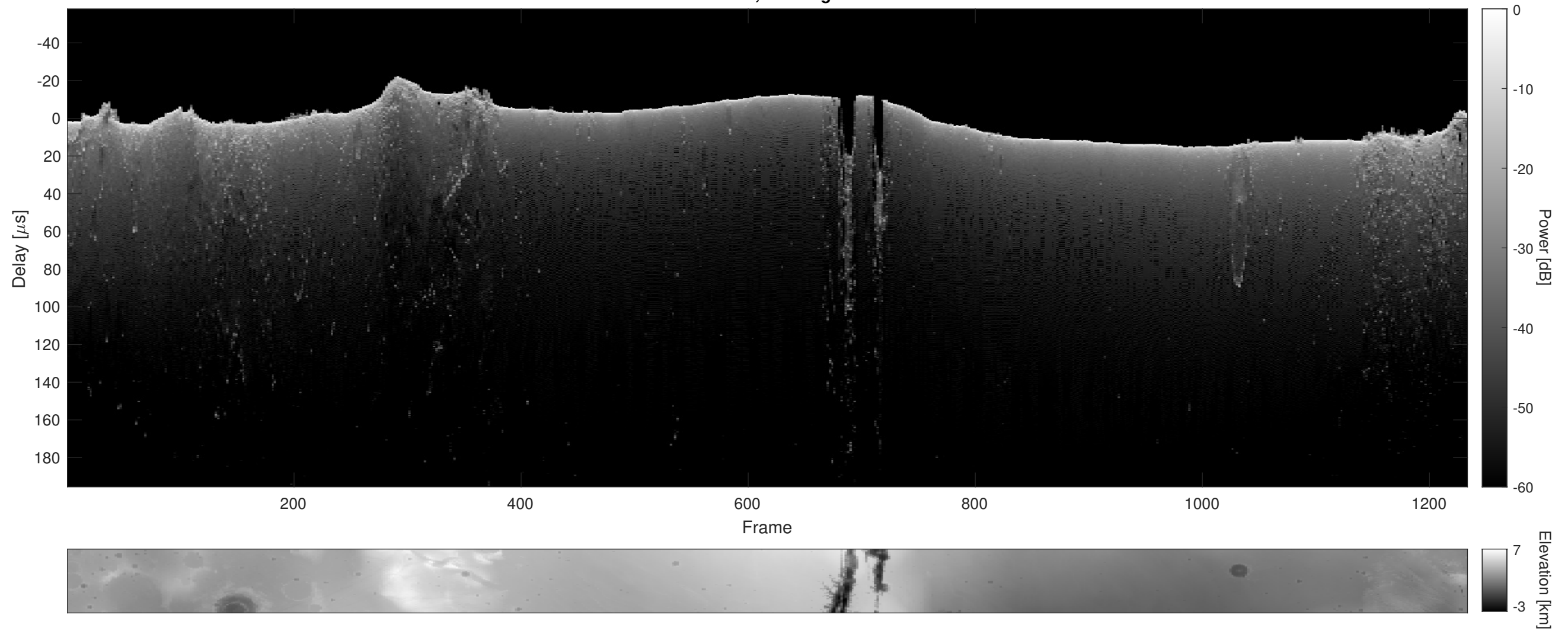
Orbit 4153, Cluttergram
