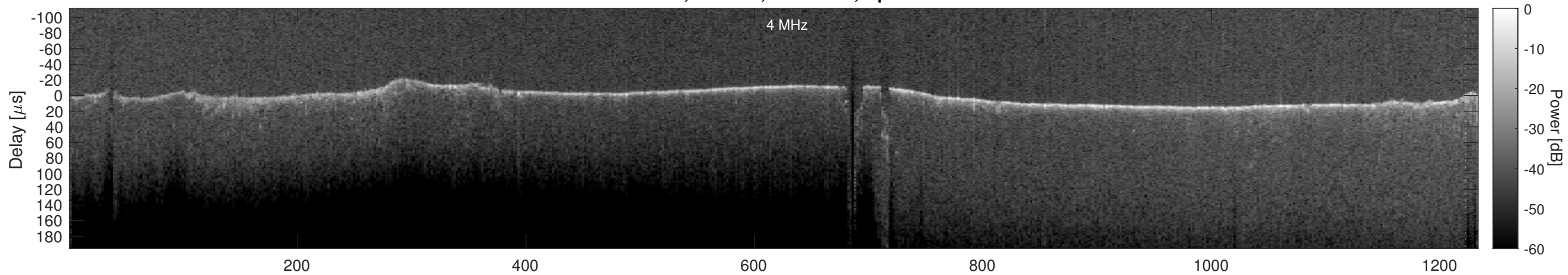
Orbit 4153, Cluttergram
