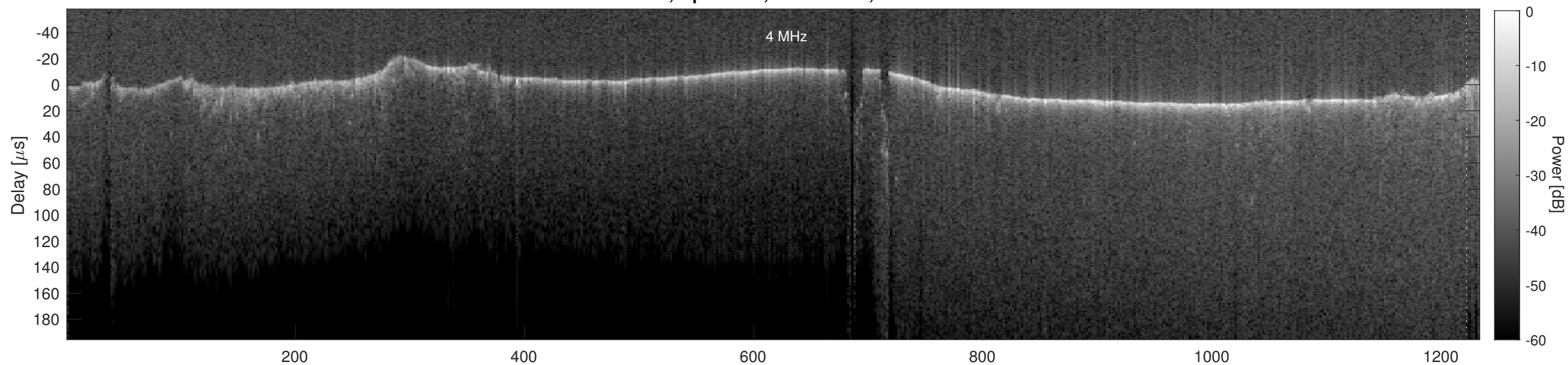
Orbit 4153, Cluttergram
