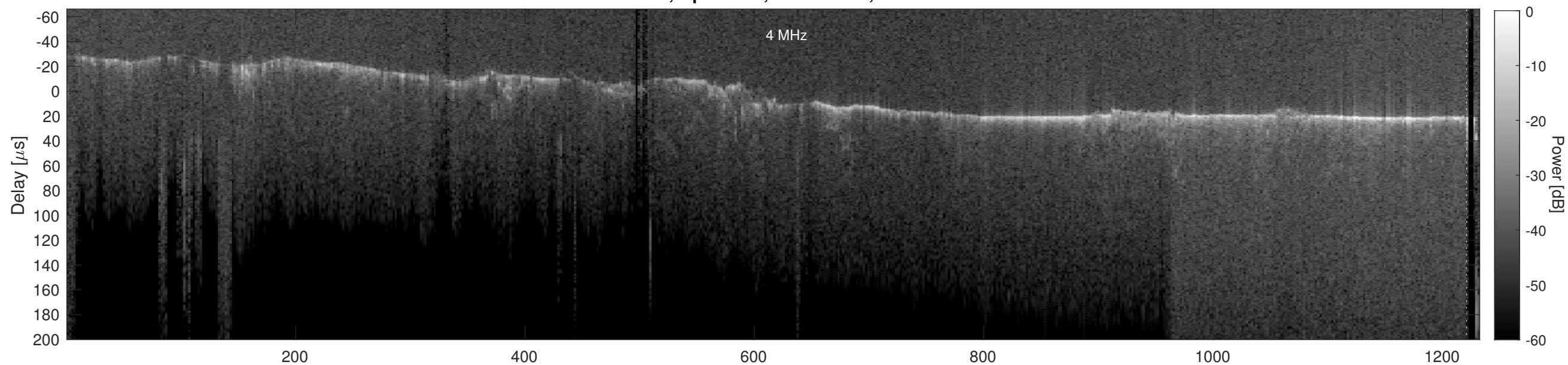
Orbit 4154, Cluttergram
