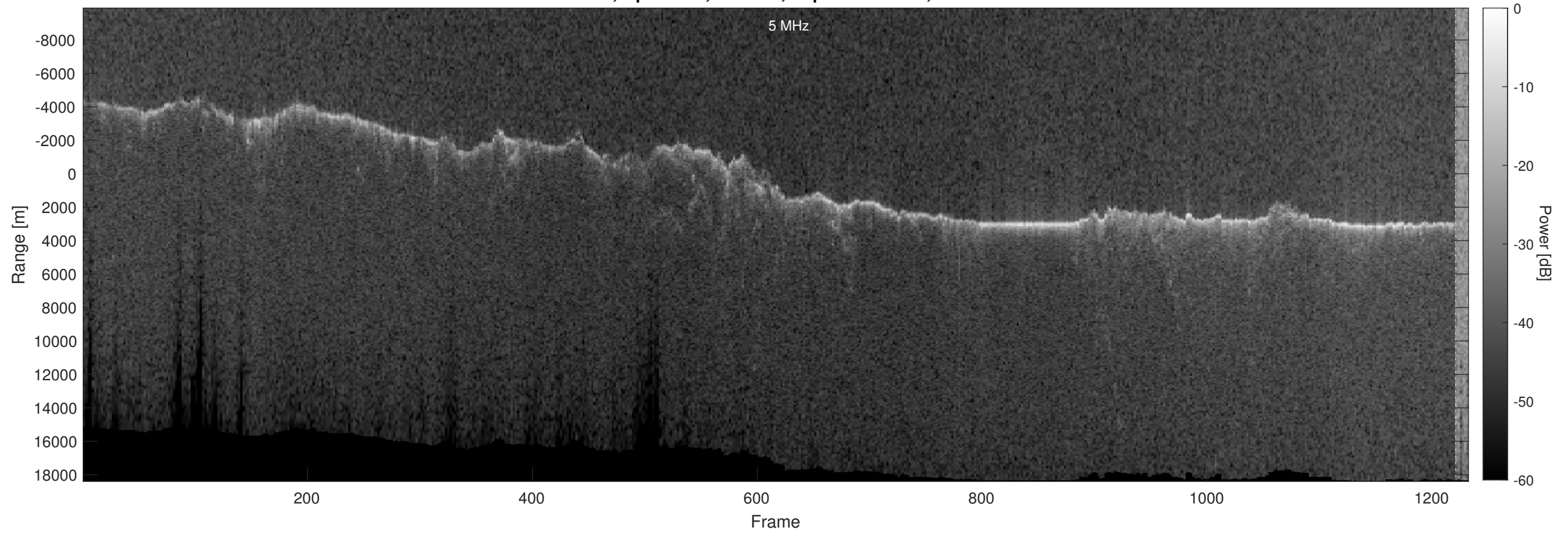
Orbit 4154, Optimized, Window, Depth-Corrected, Channel 2
