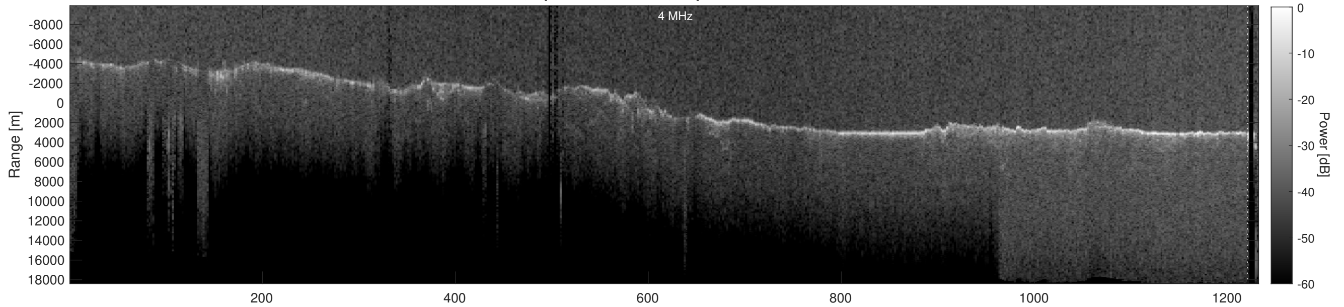
Orbit 4154, Depth-Corrected Cluttergram
