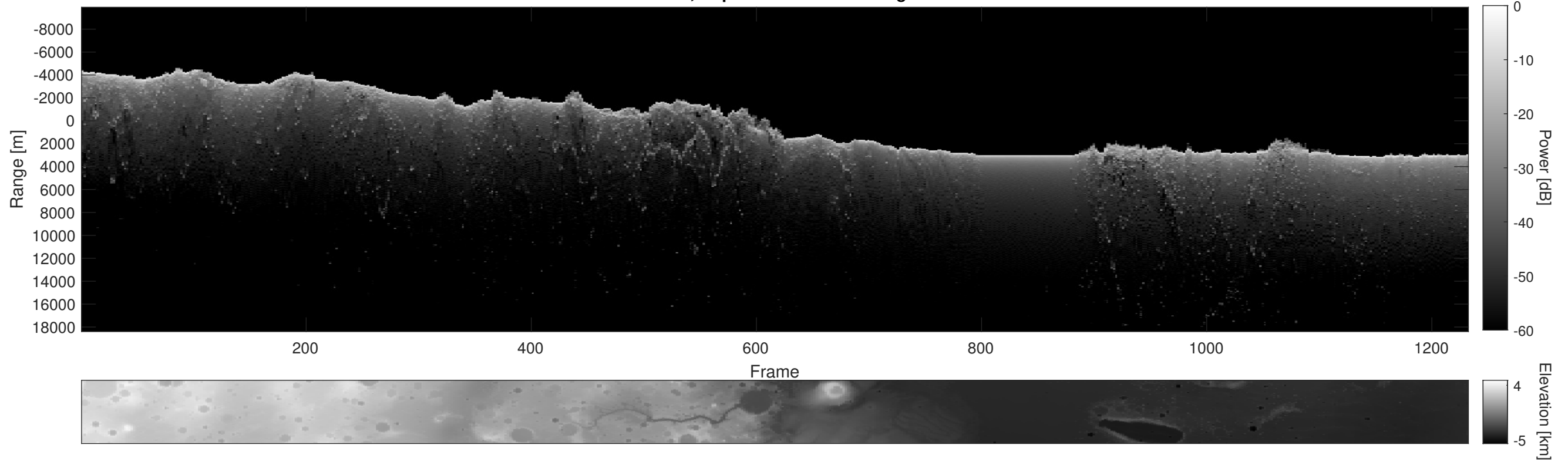
Orbit 4154, Depth-Corrected Cluttergram
