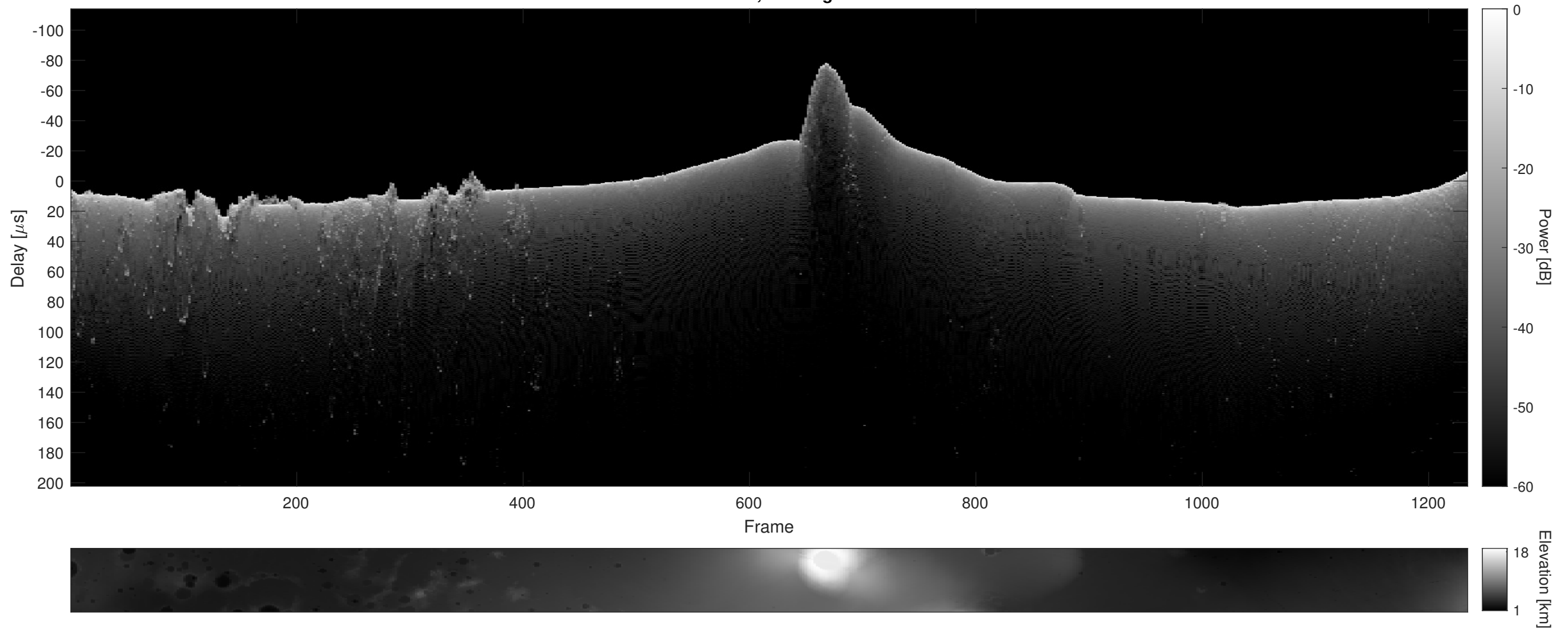
Orbit 4157, Cluttergram
