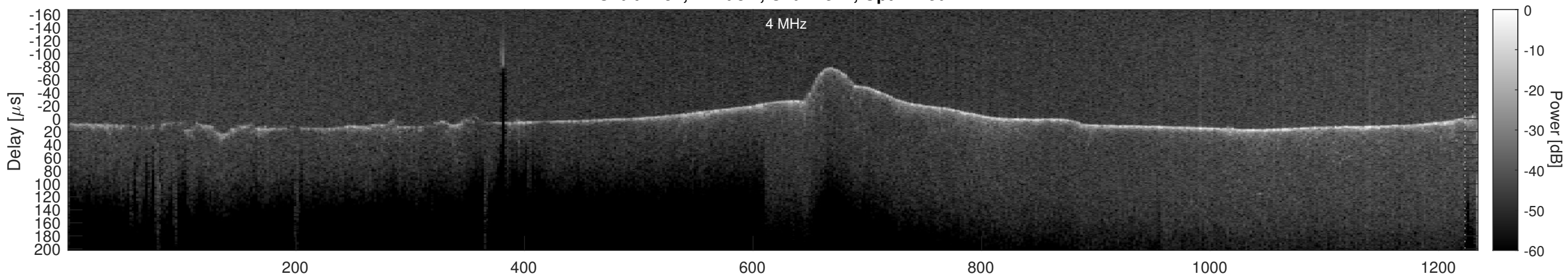
Orbit 4157, Cluttergram
