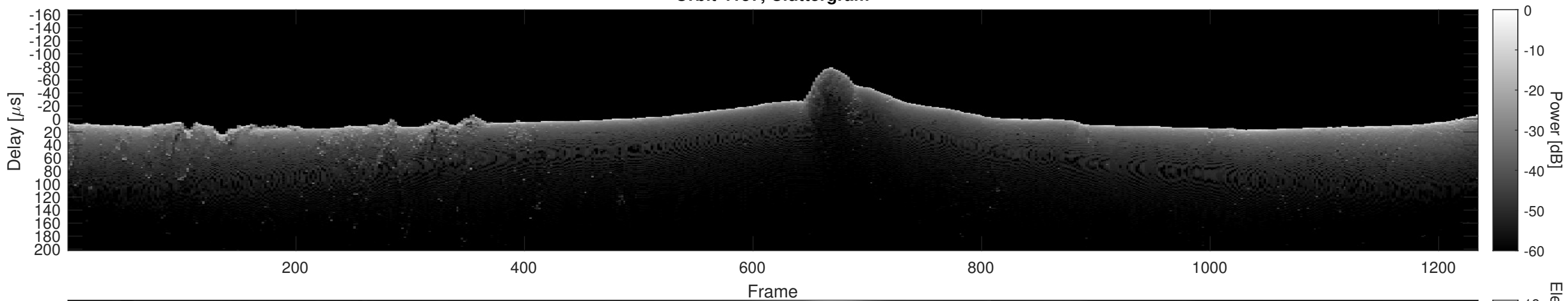
Orbit 4157, Cluttergram
