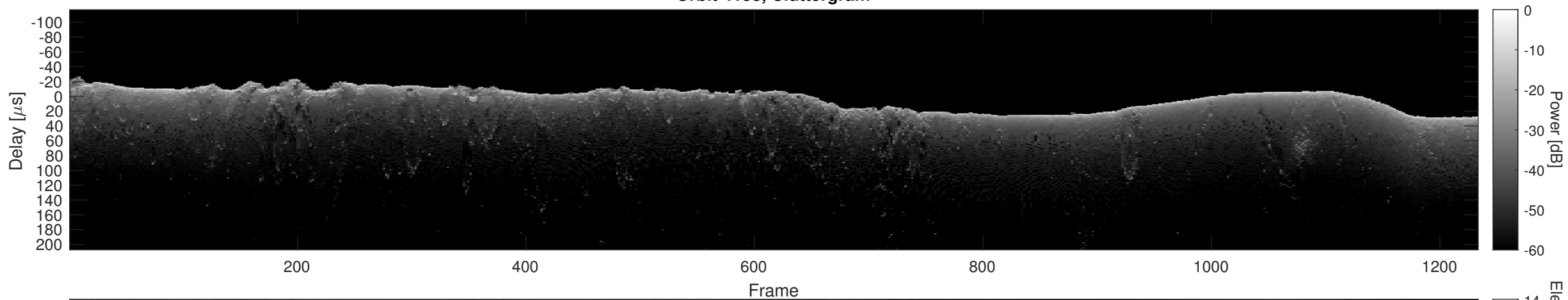
Orbit 4158, Cluttergram
