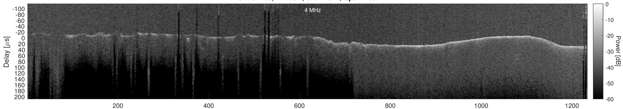
Orbit 4158, Cluttergram
