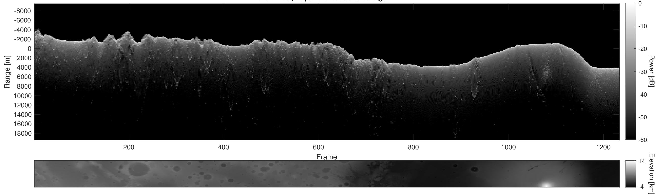
Orbit 4158, Depth-Corrected Cluttergram
