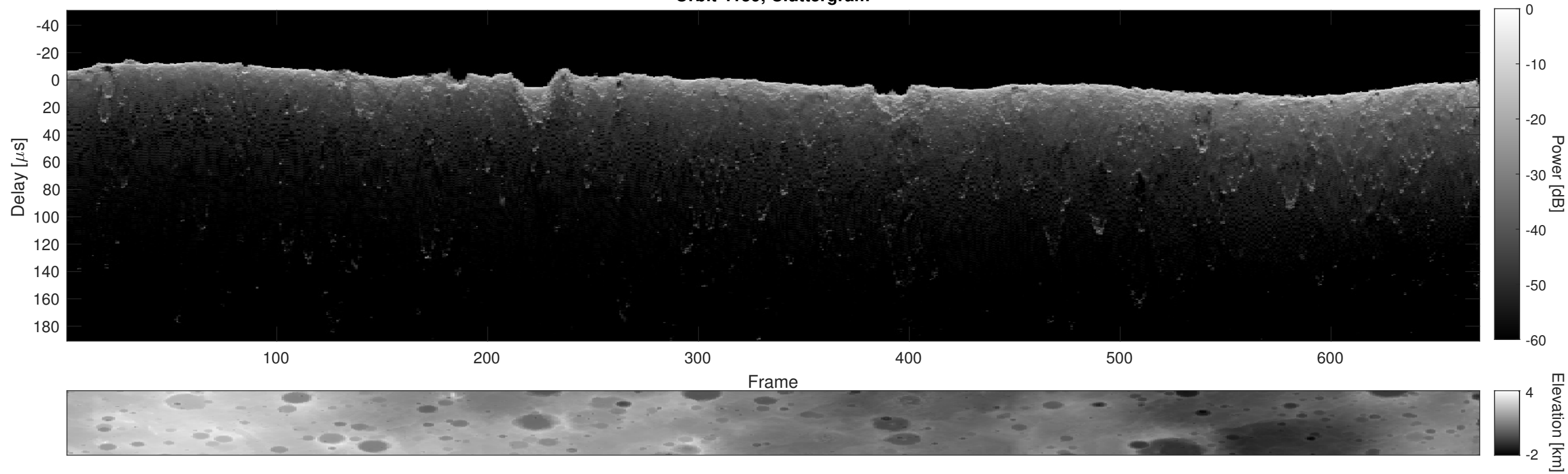
Orbit 4159, Cluttergram
