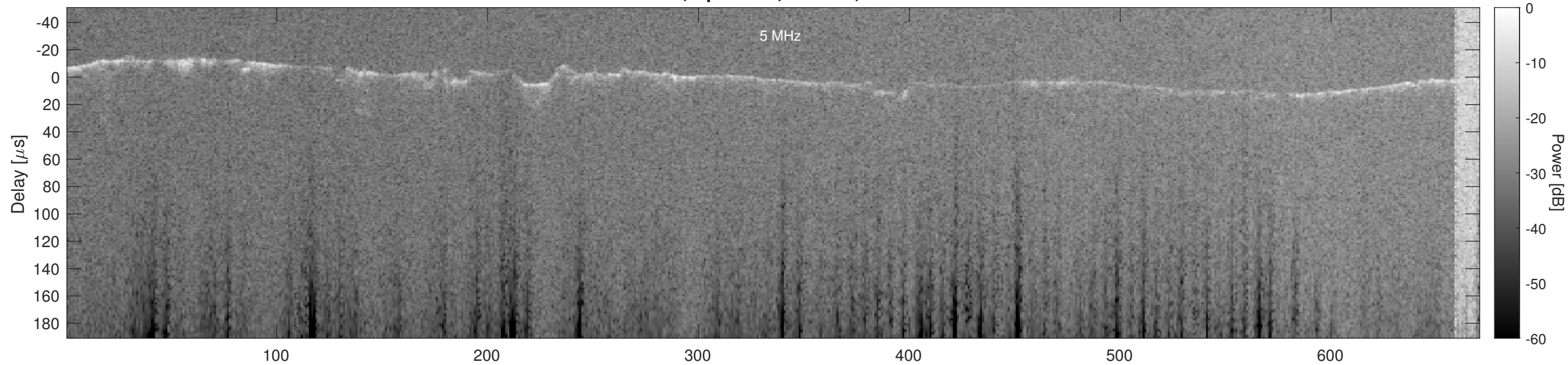
Orbit 4159, Optimized, Window, Channel 2
