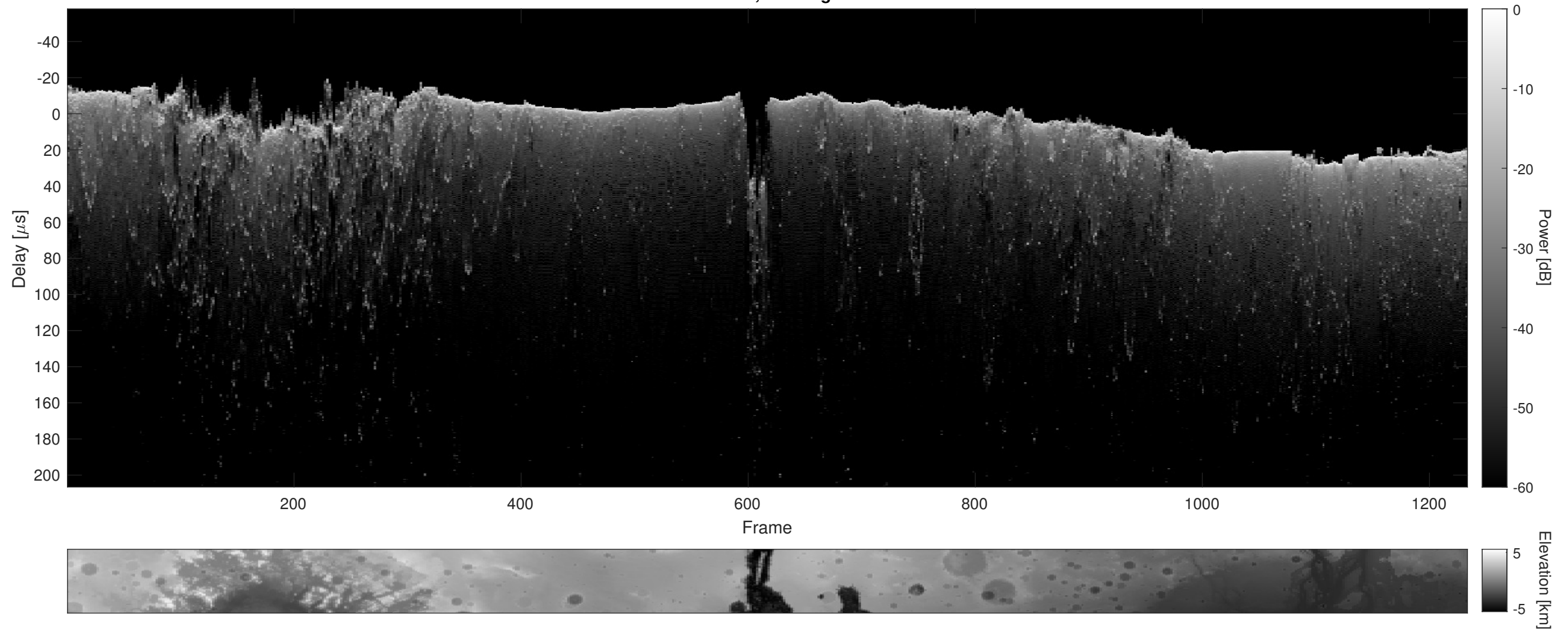
Orbit 4160, Cluttergram
