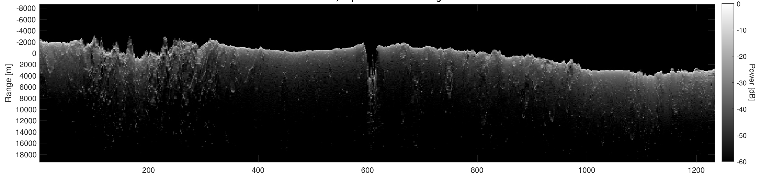
Orbit 4160, Depth-Corrected Cluttergram
