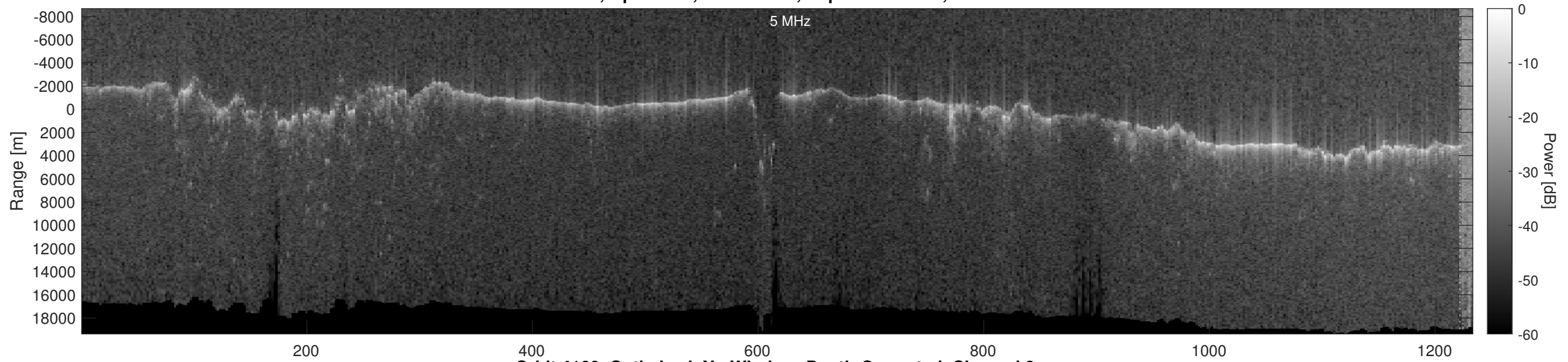
Orbit 4160, Optimized, No Window, Depth-Corrected, Channel 2
