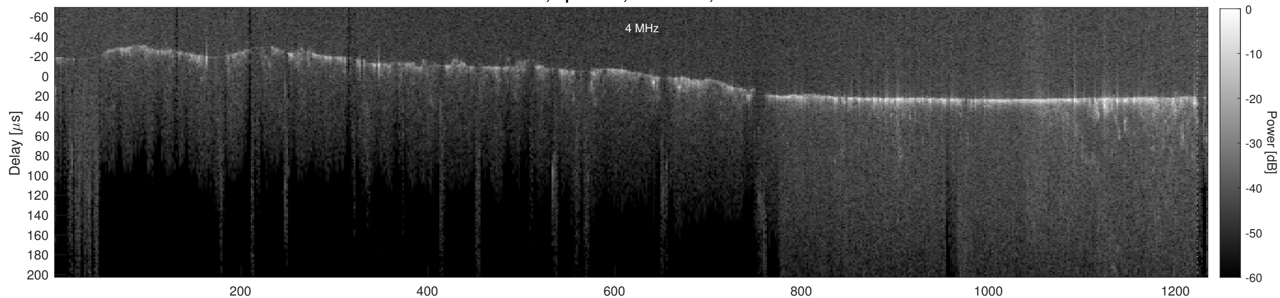
Orbit 4161, Cluttergram
