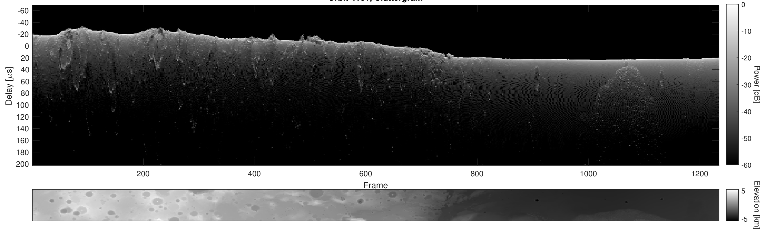
Orbit 4161, Cluttergram
