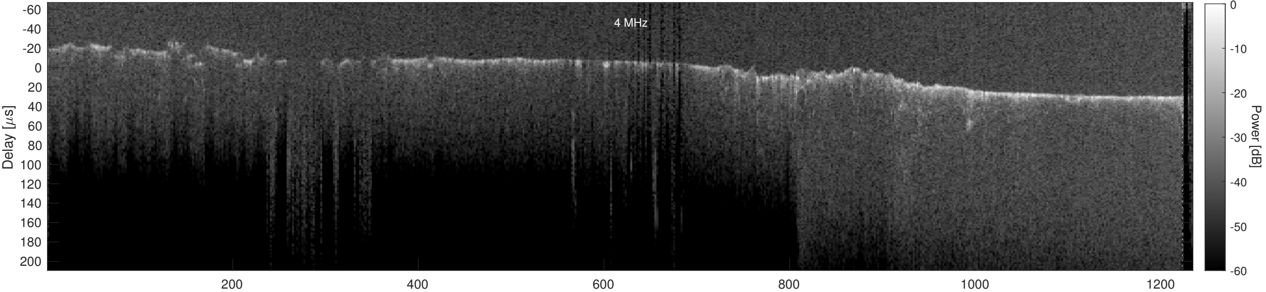
Orbit 4162, Cluttergram
