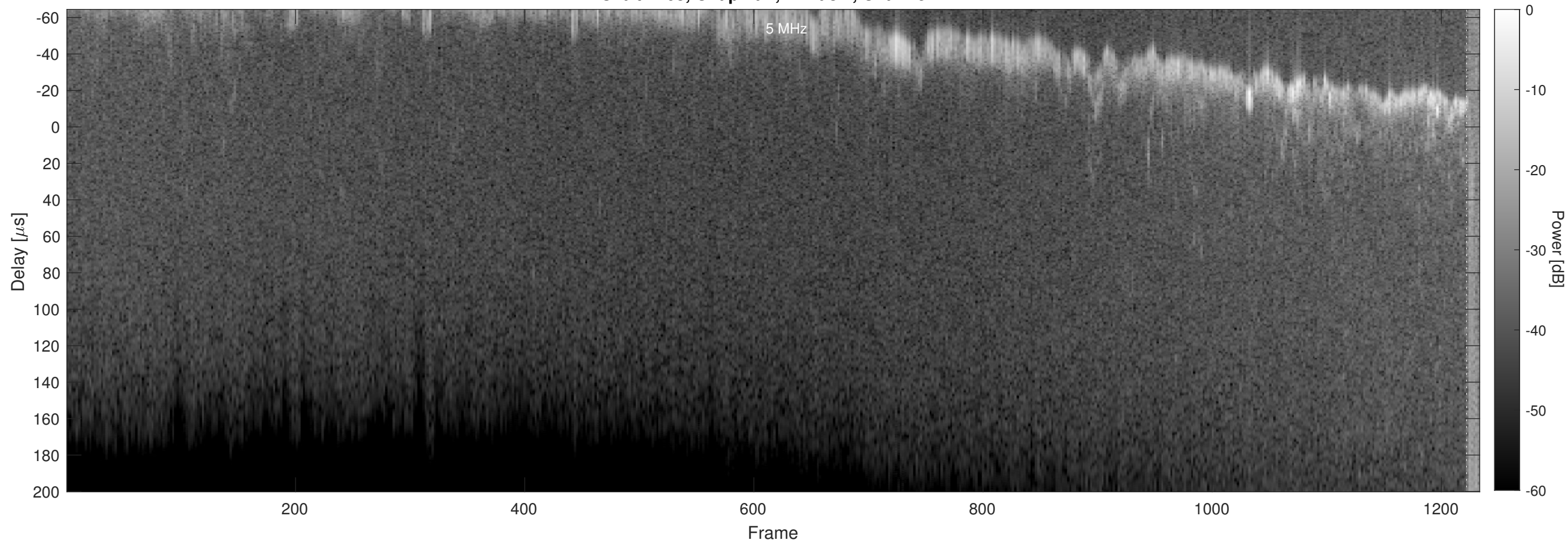
Orbit 4163, Chapman, Window, Channel 2
