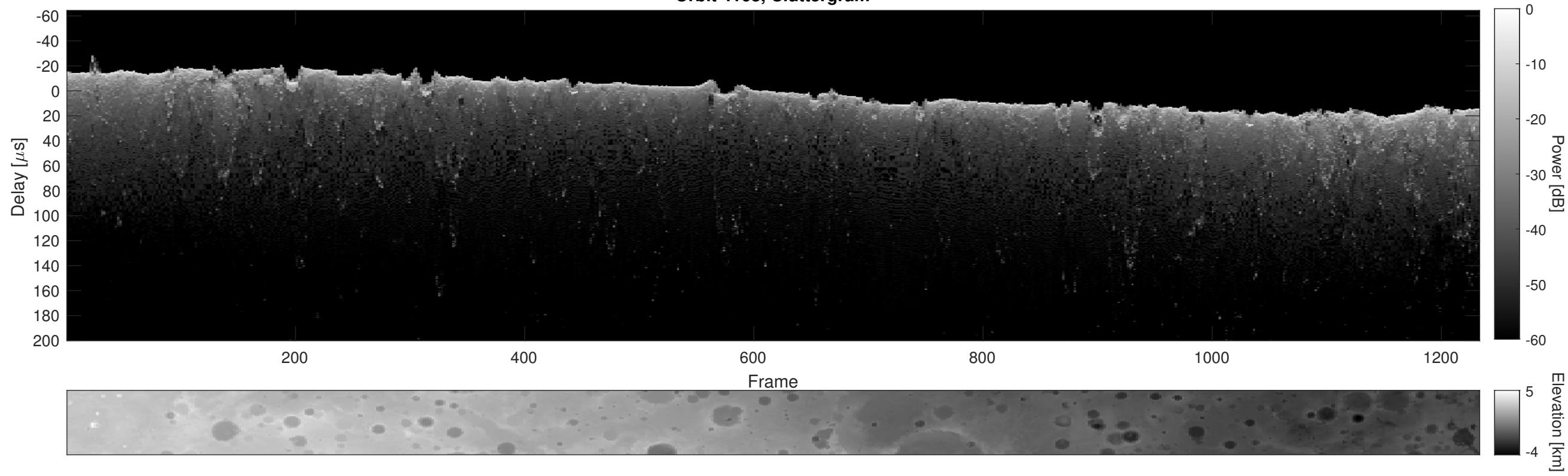
Orbit 4163, Cluttergram
