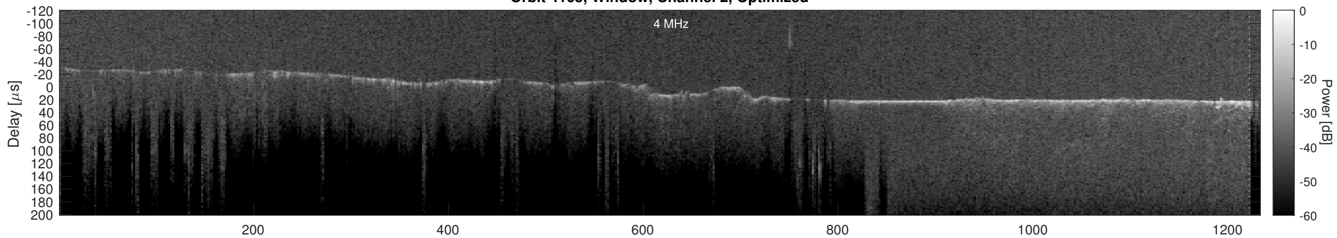
Orbit 4165, Cluttergram
