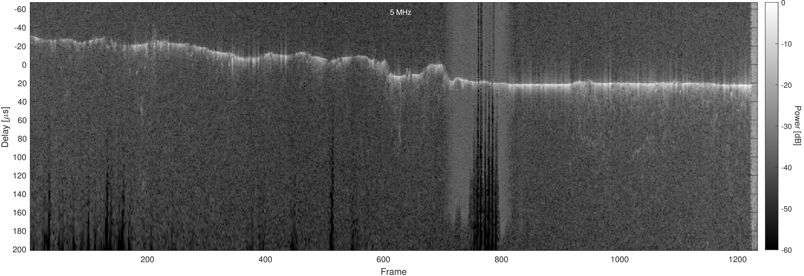
Orbit 4165, Optimized, No Window, Channel 2
