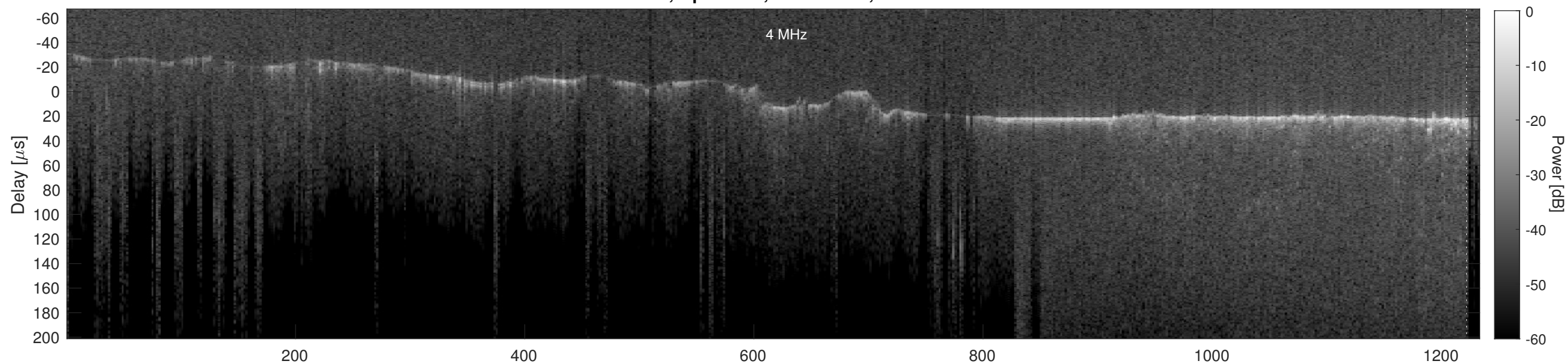
Orbit 4165, Cluttergram
