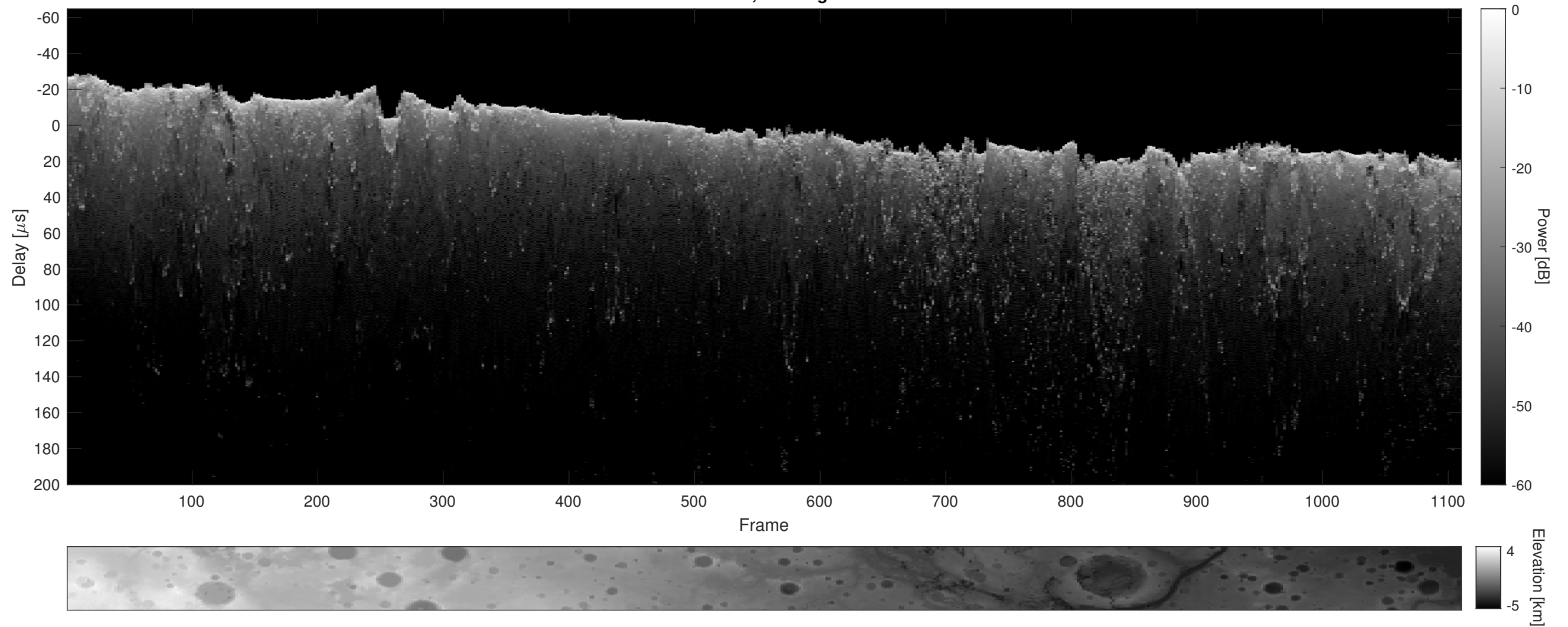
Orbit 4167, Cluttergram
