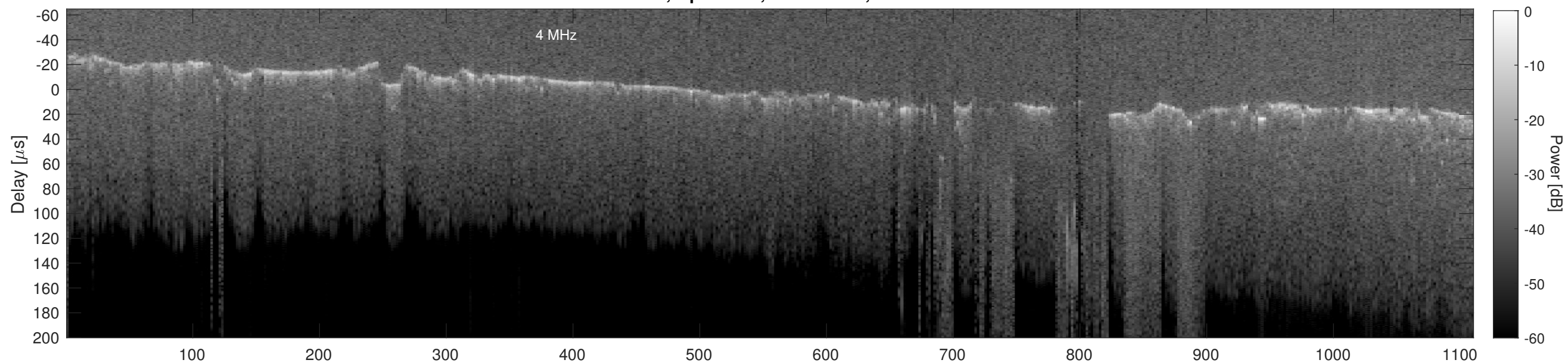
Orbit 4167, Cluttergram
