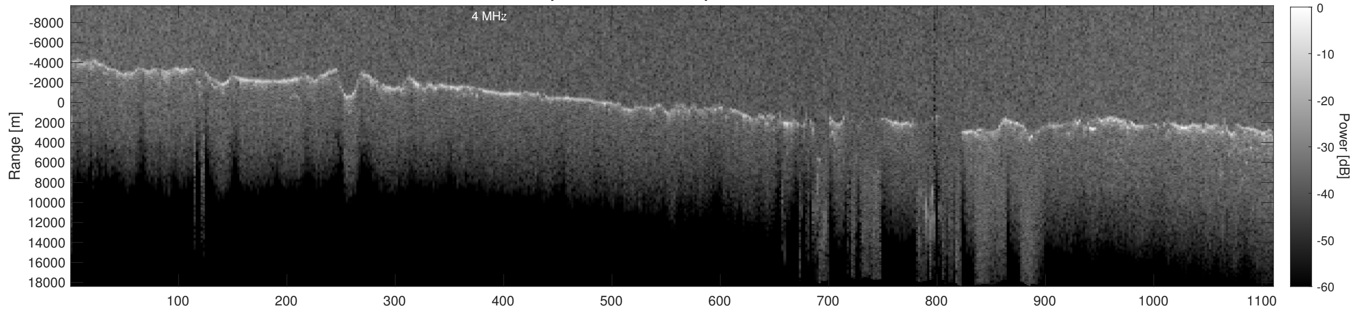
Orbit 4167, Depth-Corrected Cluttergram
