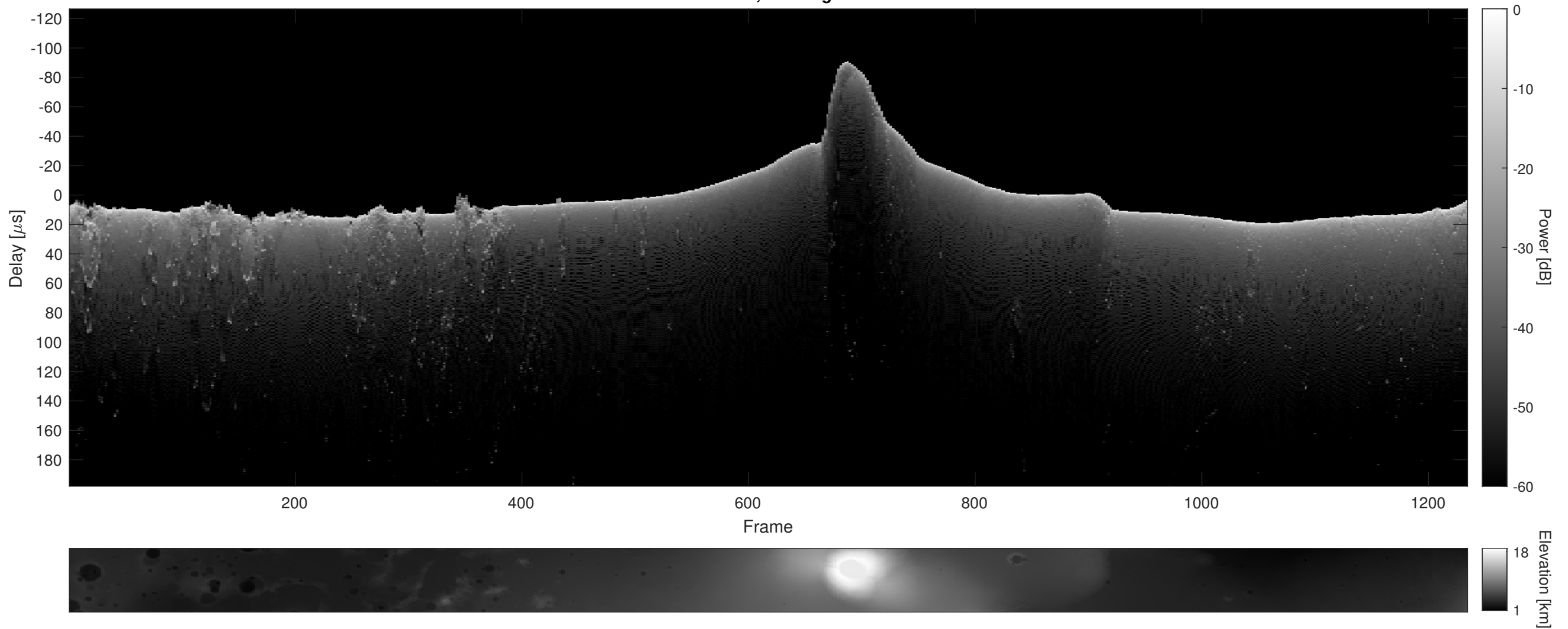
Orbit 4168, Cluttergram
